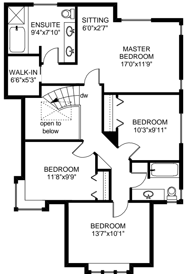
UPPER FLOOR 1050 SQ.FT
