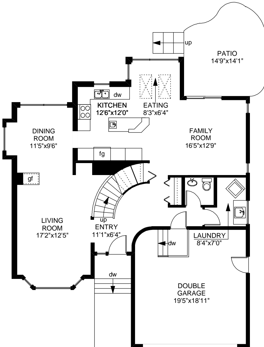
MAIN FLOOR 1168 SQ.FT
